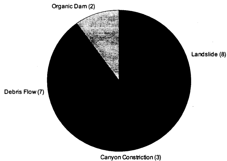
Fig. 3.1 Number of dam-break sites and corresponding initiation modes.
