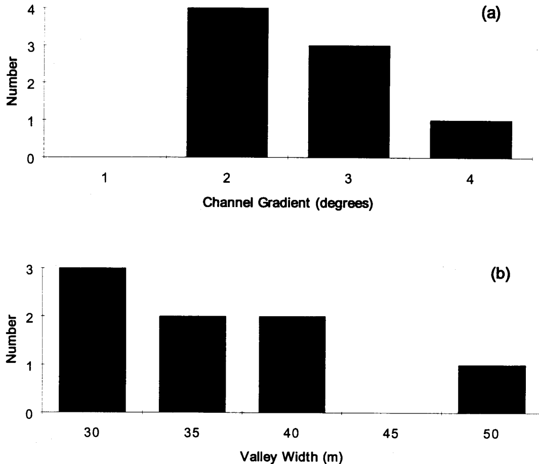
Fig. 3.5 Number of dam-break deposition sites with respect to (a) channel slopes (class interval 1^\circ ), and (b) valley widths (class interval 5 m), ( n = 8 ).
