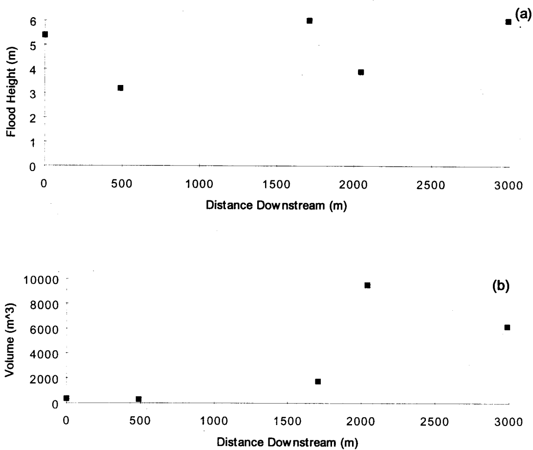
Fig. 4.11 (a) Flood height and (b) estimated volume of impounded water as a function of distance from the initiation site along Twin Creek.
