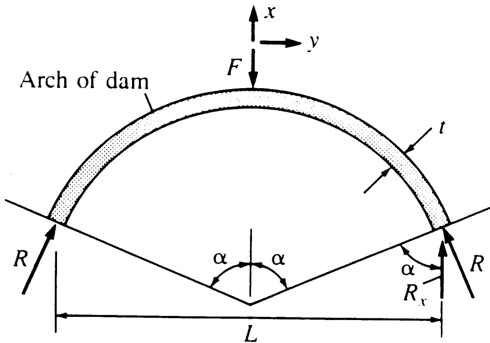
Fig. 5.2 Plan view of arch dam showing applied hydrostatic force F and the resulting force R from each abutment transmitted to the arch structure.
