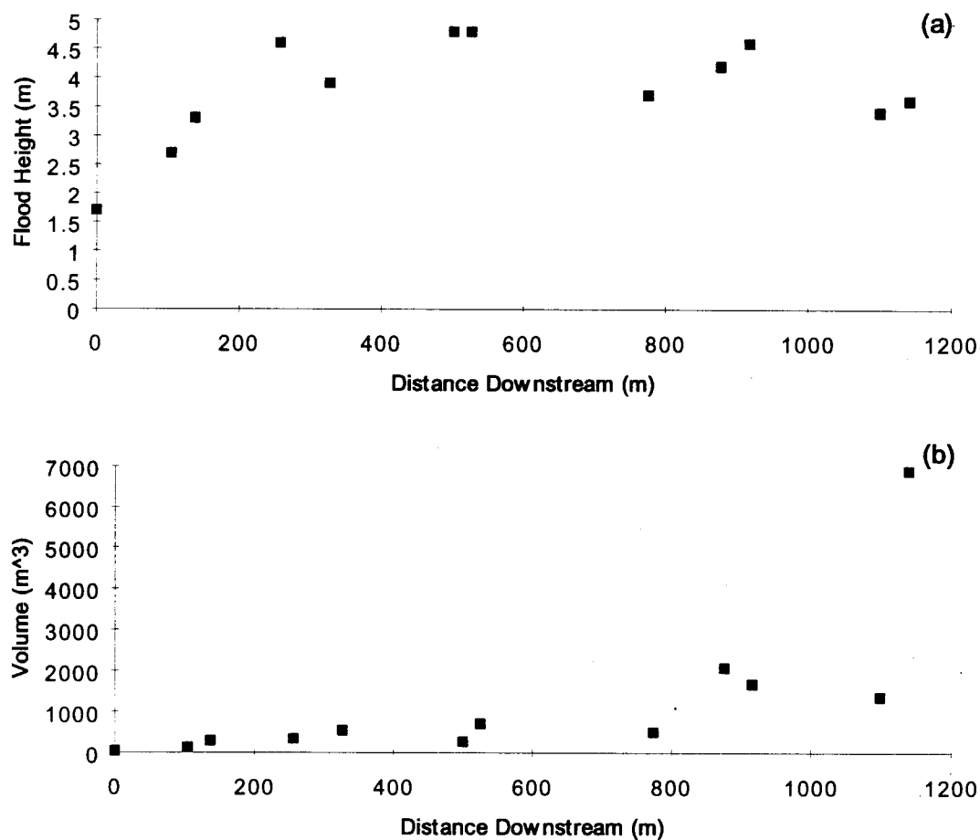
Fig. 4.16 (a) Flood height and (b) estimated volume of impounded water as a function of distance from the initiation site along Ware Creek.
