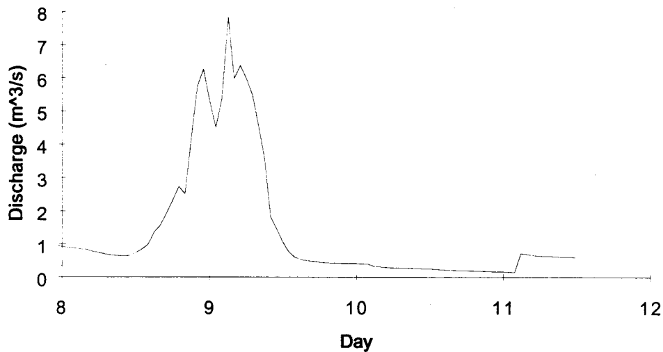
Fig. 4.15 Estimated hydrograph of Ware Creek in the absence of debris dam failure, January 8-12, 1990; gauge location shown in Figure 4.12.
