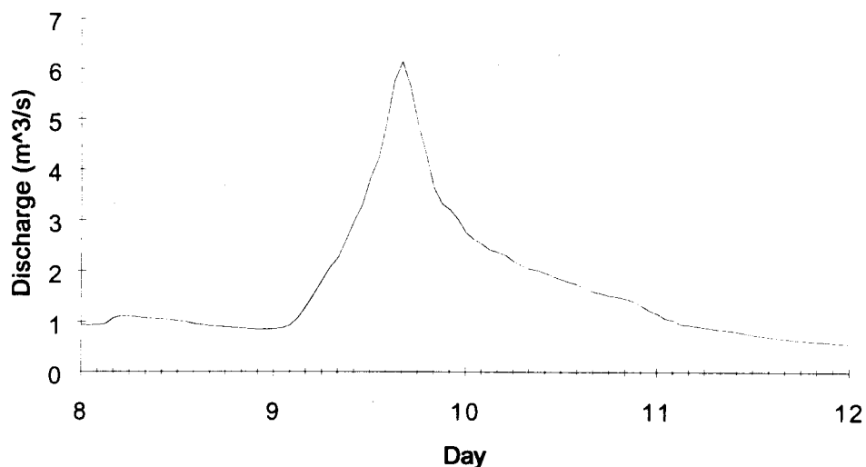
Fig. 4.7 Estimated downstream hydrograph of Huckleberry Creek in the absence of debris-dam failure for January 8-12, 1990; gauge location shown in Figure 4.4.
