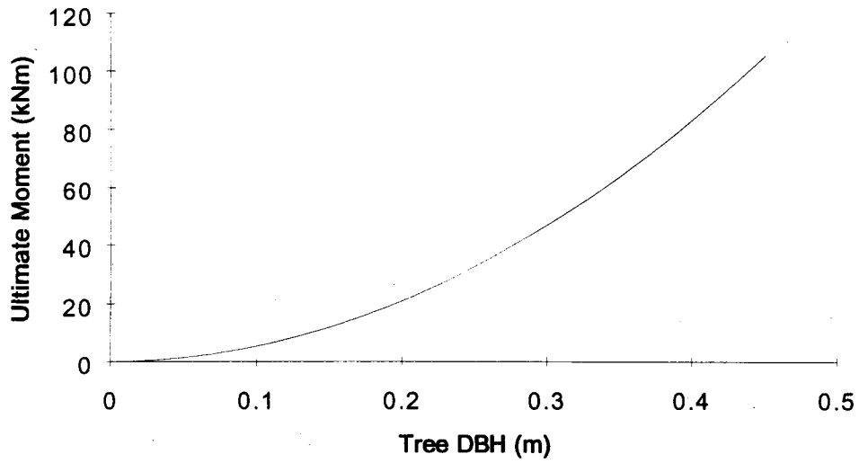
Fig. 5.6 Relationship between ultimate breaking moment and tree diameter breast height (DBH).
