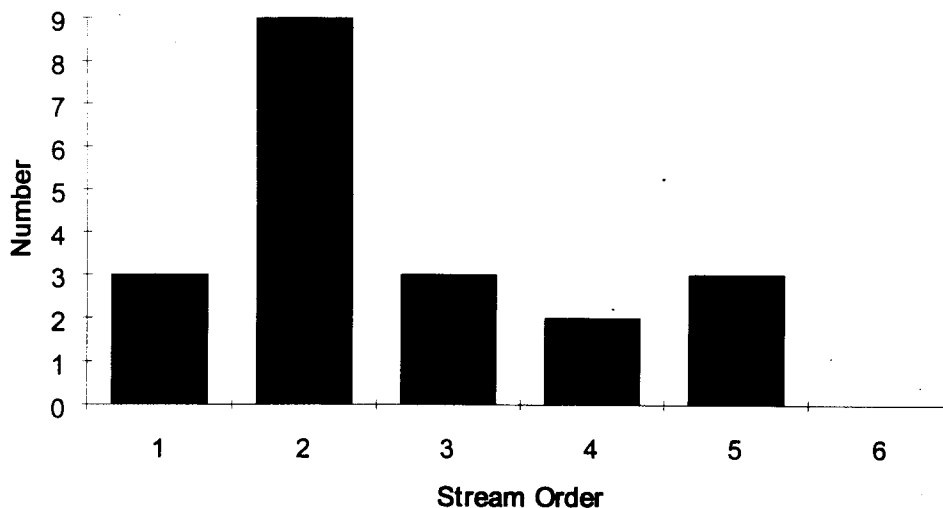
Fig. 3.4 Number of streams of order m where dam-break initiation occurred ( n = 20 ).
