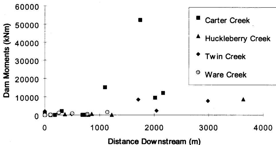
Fig. 5.9 Calculated dam moments as a function of distance downstream from the initiation point.
