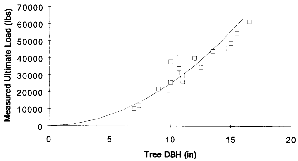
Fig. 5.5 Relationship between ultimate load and tree diameter breast height (DBH).
