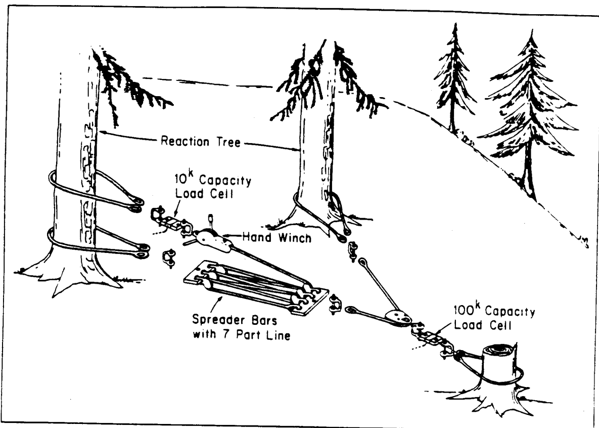
Fig. 5.4 Schematic diagram of Pyles' experiment in which ultimate static loads on tree stumps were measured (load applied 1 ft. above ground surface).
