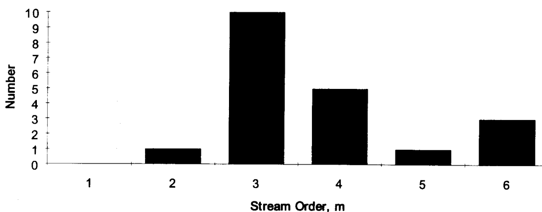
Fig. 3.6 Number of streams of order m where dam-break deposition occurred ( n=20 ).
